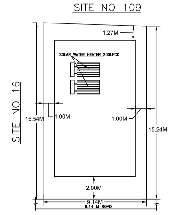
SITE PLAN
